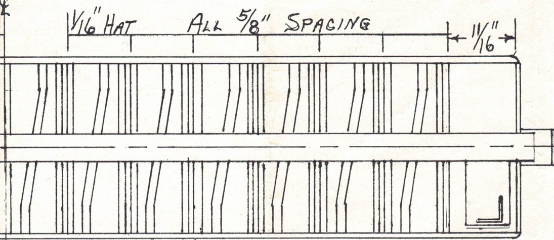
ROOF "B" (SEE EXPLODED VIEW)
