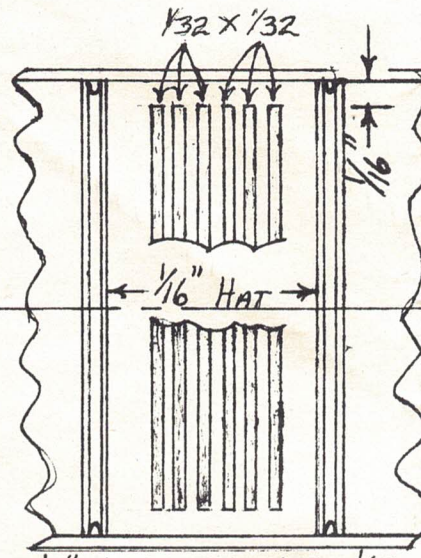
EXPLODED VIEW ROOF "A" (NOT TO SCALE)
