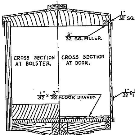
KIT SB-5. SHEET NO. 1. 3 GAUGE. VENTILATED BOX CAR NORTHEASTERN SCALE MODELS BOX 32 ANDOVER, MASS.
