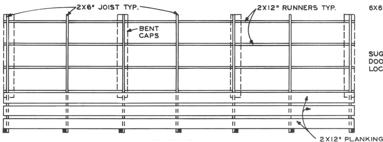
TANK FRAME TEMP.
