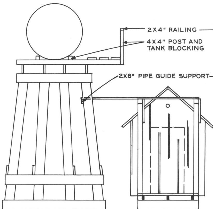
LEFT SIDE VIEW AND TEMPLATES
