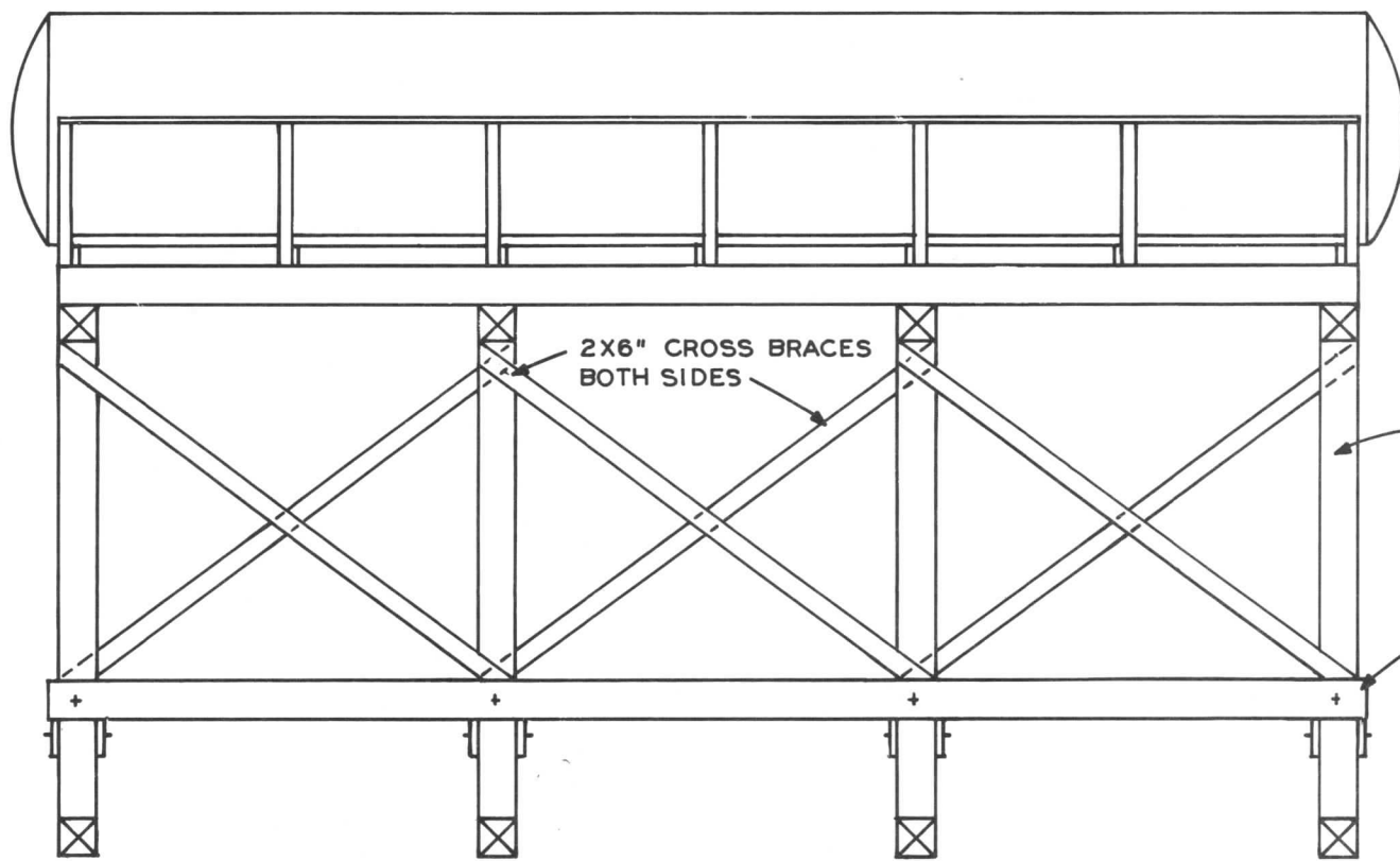
FRONT VIEW
