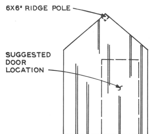
PUMPHOUSE END WALLS
