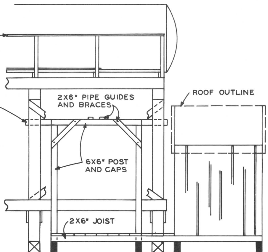
PUMPHOUSE AND PLATFORM FRONT VIEW
