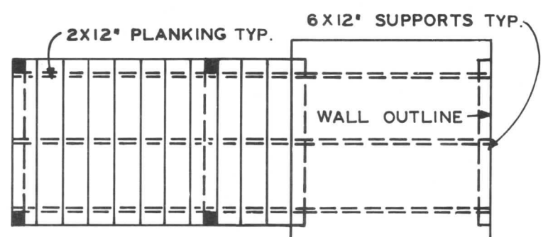
PLATFORM FRAMING TEMP.
